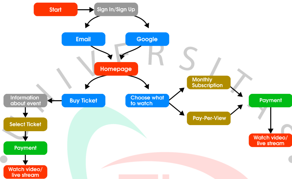
Lampiran 1 9 User Flow
