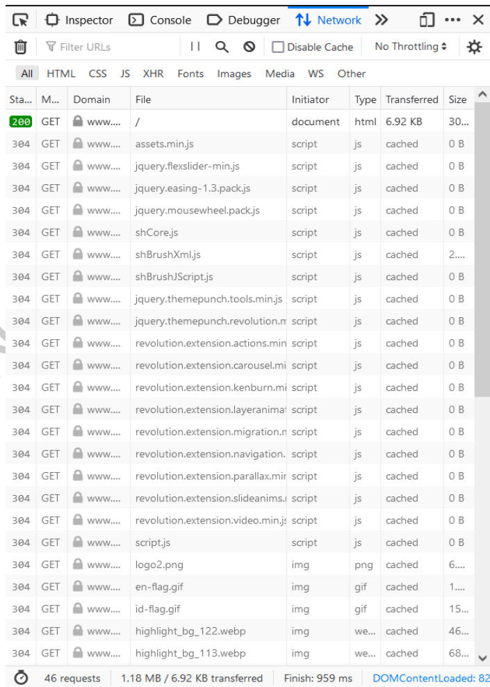
Gambar 3. 18 Mozilla Firefox Networking Tools
