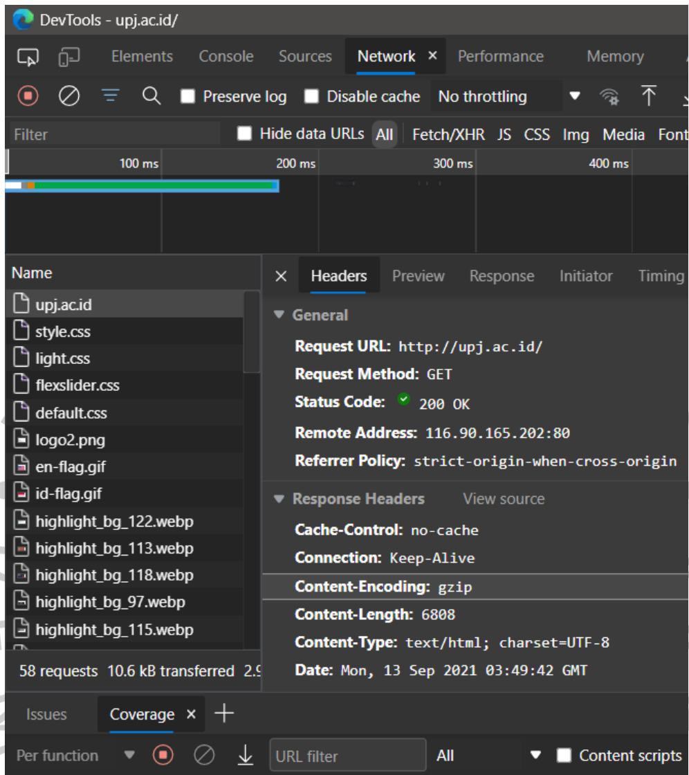
Gambar 3. 17 Microsoft Edge Network Tools
