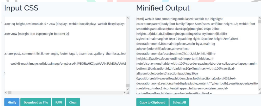
Gambar 3. 23 CSS Minifier
