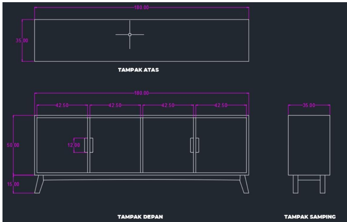
Lampiran 2.14. Gambar Kerja Custom Product
