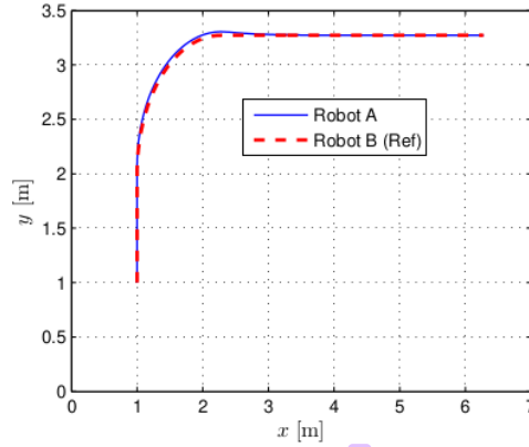
Fig. 4. The trajectory tracking performance of the TWR-A with respect to the TWR-B in the first simulation, where an initial posture of both TWRs are identical.
