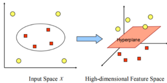
Fig. 2: Geometrical representation of Kernel.
