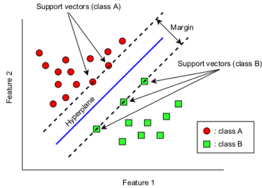
Fig. 1: An illustration of the SVM concept.
