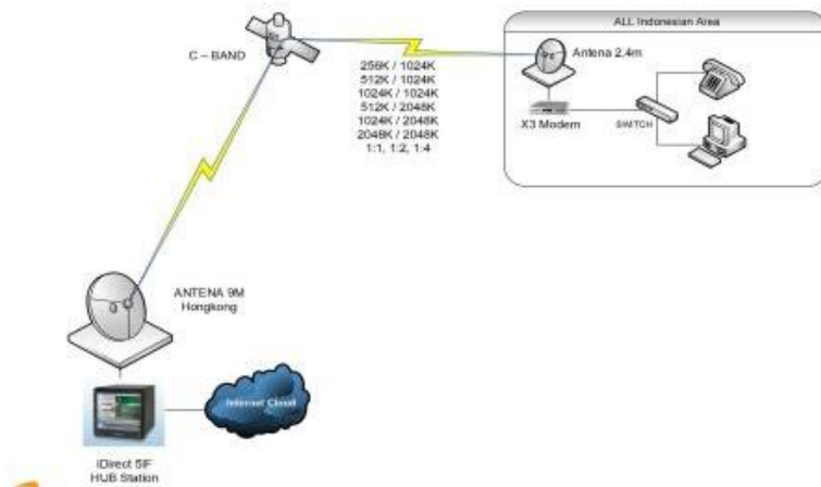
Gambar 2.5 VSAT C-Band Premium Internet
