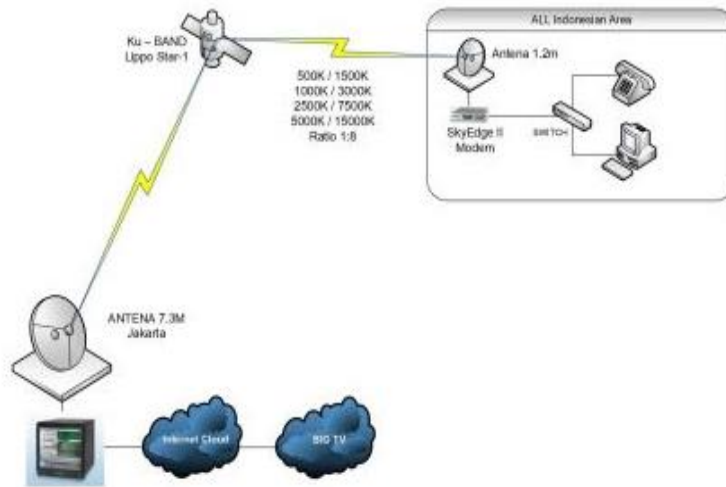
Gambar 2.6 VSAT Ku-Band Combo Premium Internet + HDTV
