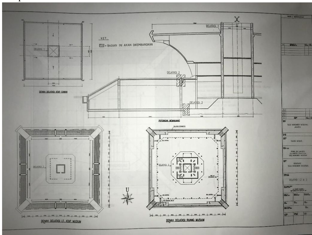
Lampiran 5 Denah Delatasi
