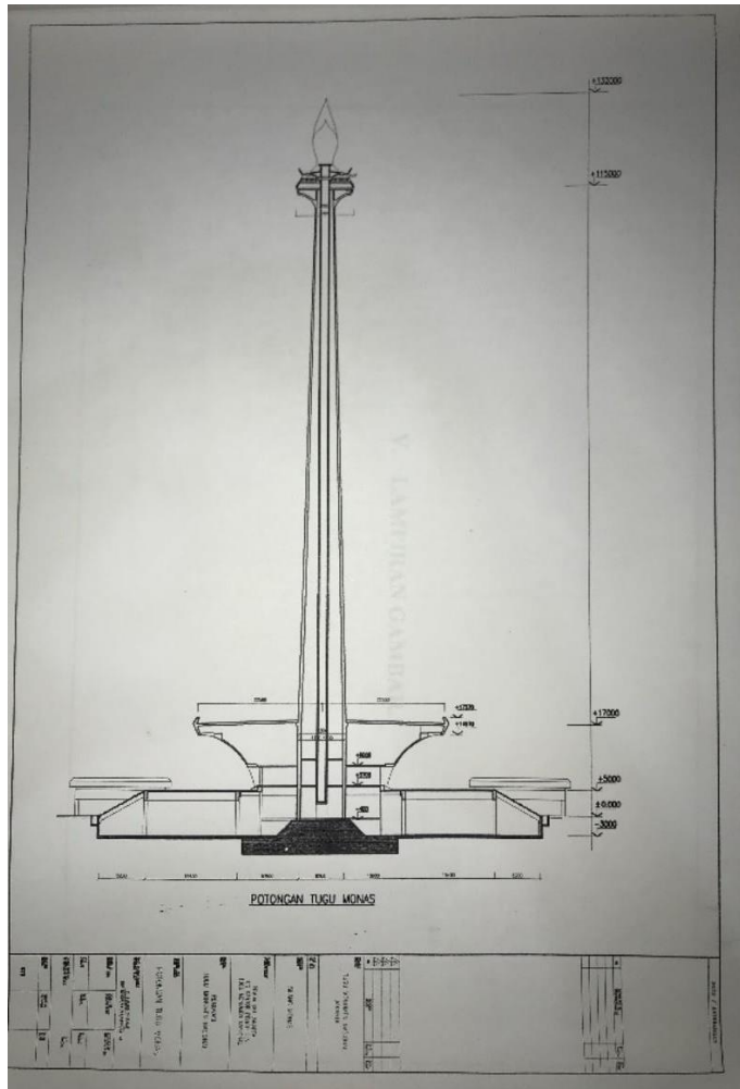
Lampiran 1 Potongan Tugu Monas
