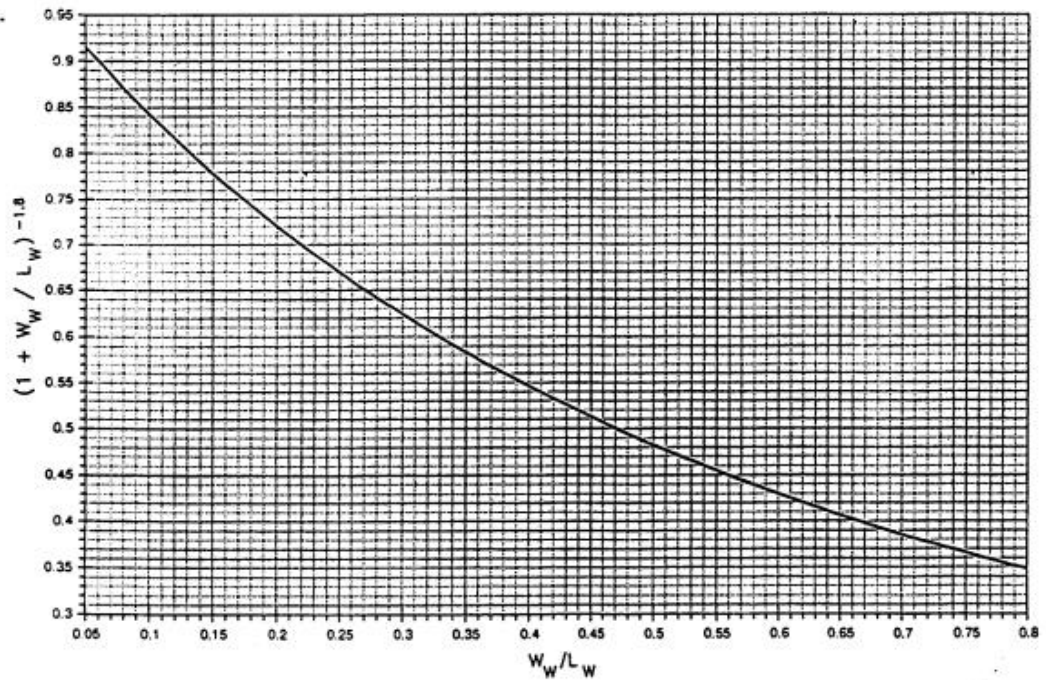
Lampiran 4 Nilai (1 + W_w/L_w)^{-1.8} Terhadap W_w/L_w
