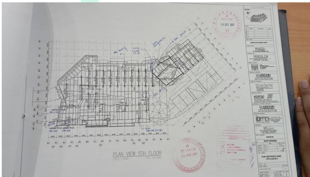
Lampiran C- 6 Gambar Shop drawing Plan View 5 th Floor.
