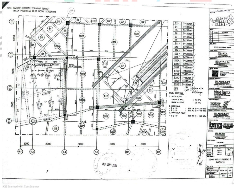
Lampiran C- 8 Gambar Shop drawing Denah Plat Lantai 4 Partial 5.
