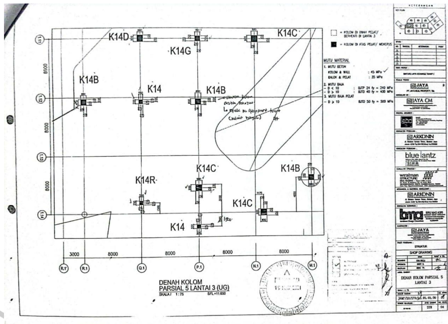
Lampiran C- 9 Gambar Shop drawing Denah Kolom Lantai 3 Partial 5.
