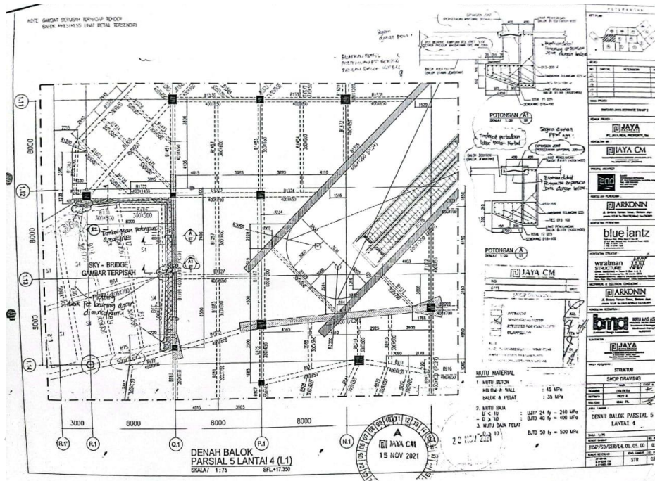
Lampiran C- 7 Gambar Shop Drawing Denah Balok Lantai 4 Partial 5.
