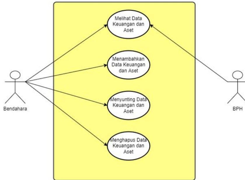
Gambar 3.6. Diagram use case.
