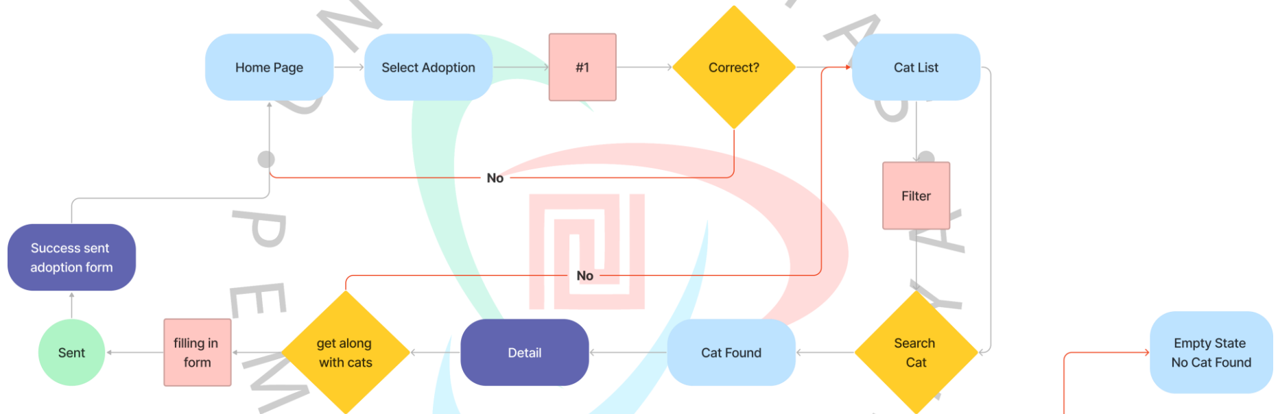
Lampiran 1. 10 User Flow Adopsi Kucing
