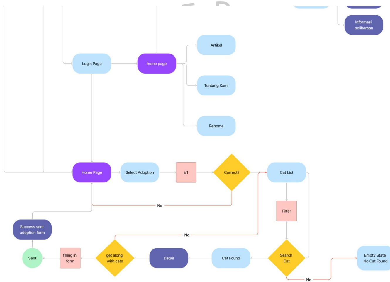
Lampiran 1. 9 User Flow Makro Adopter
