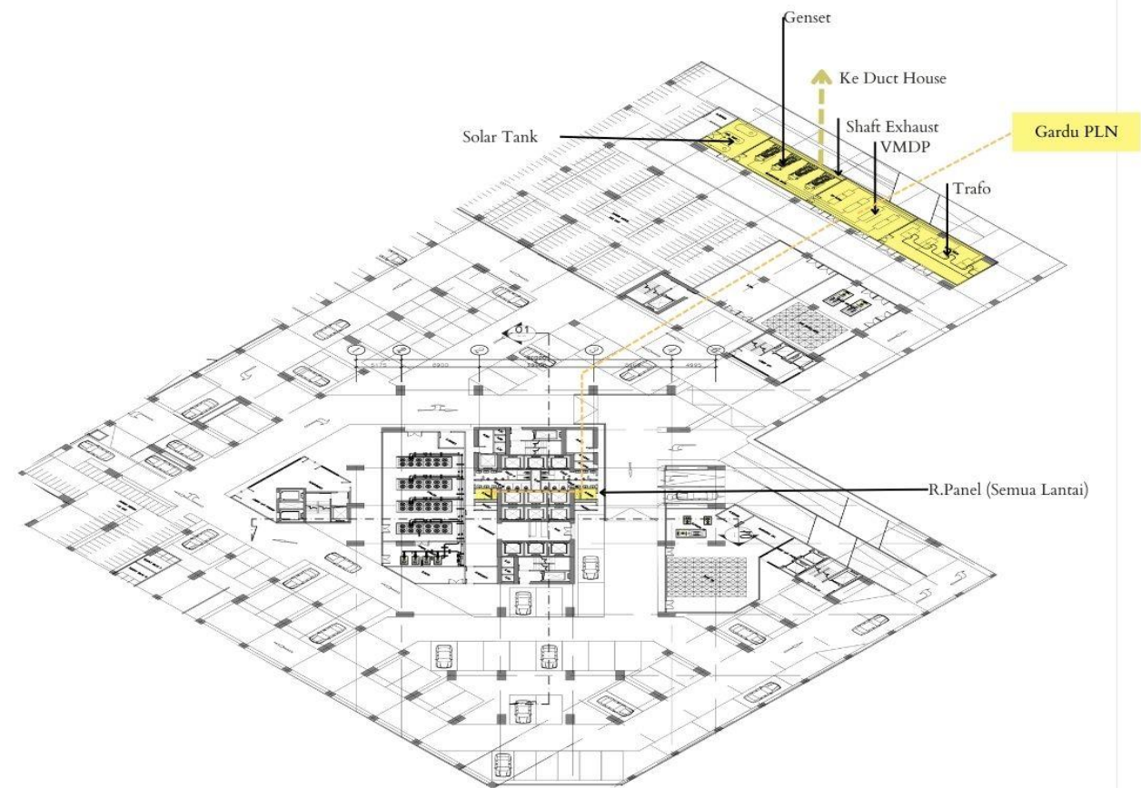
LANTAI B1
