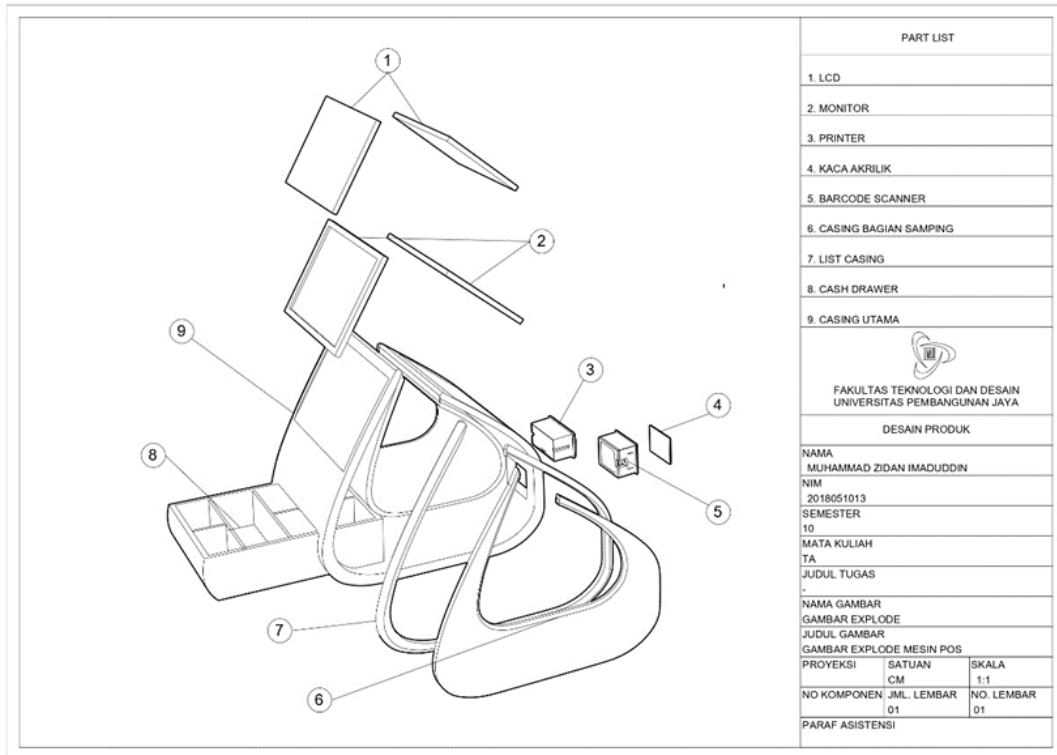
Lampiran 4. Gambar explode
