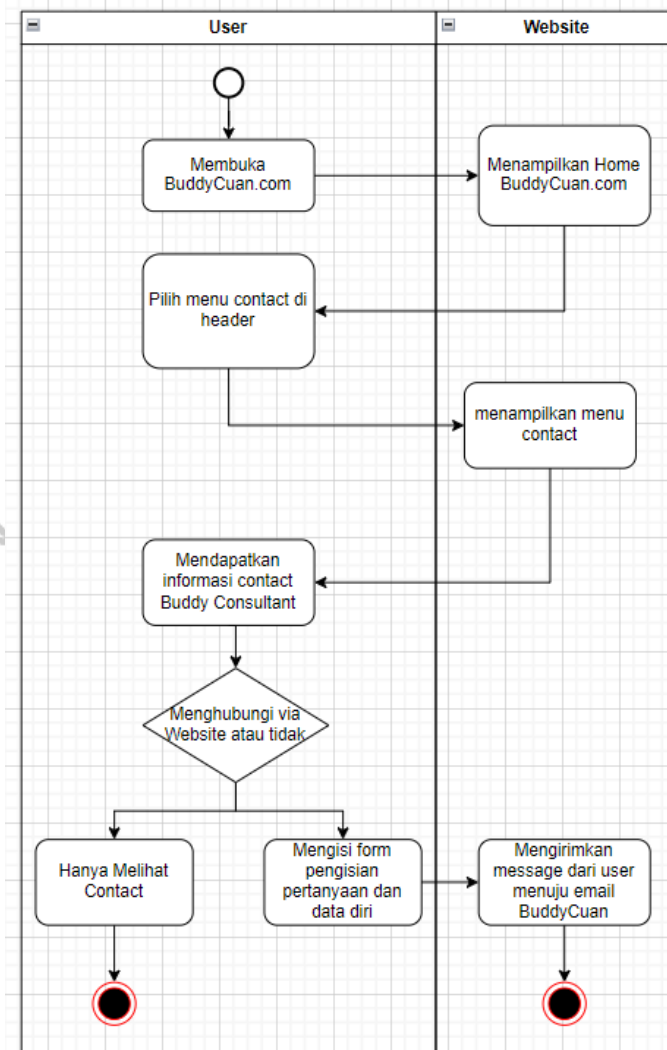
Gambar 3.3 Act Diagram Mengakses Menu Contact BuddyCuan
