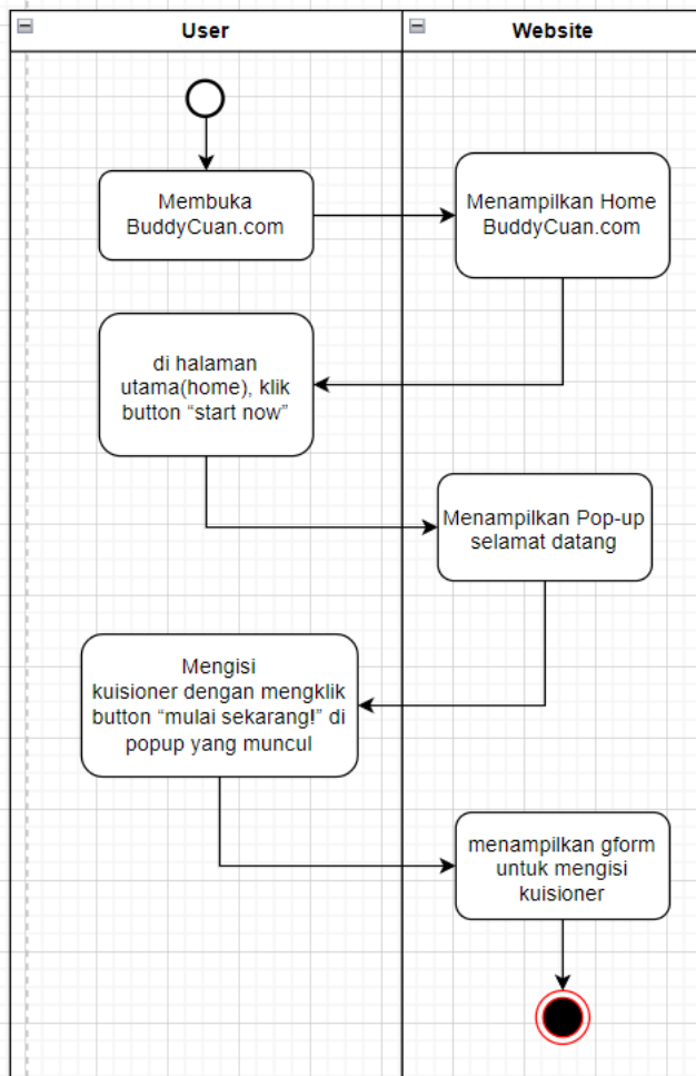
Gambar 3.4 Act Diagram Mengisi kuisisioner risk profile
