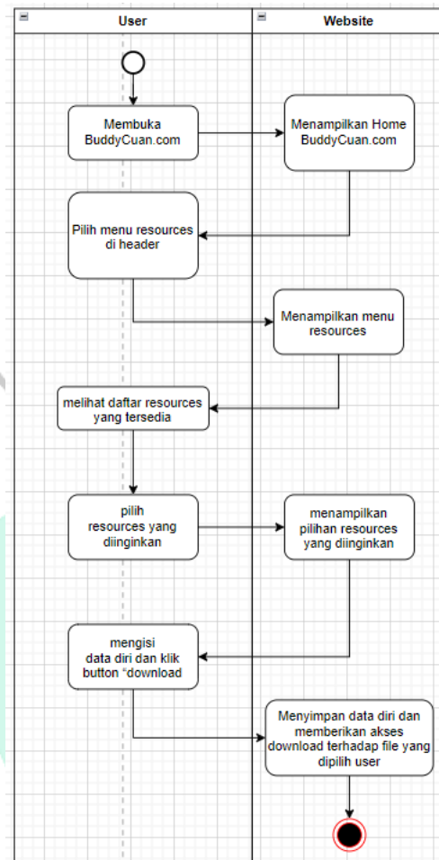
Gambar 3.9 Act Diagram Mengakses Menu Resources
