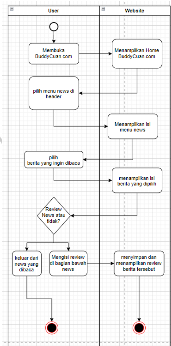
Gambar 3.5 Act Diagram Melihat News
