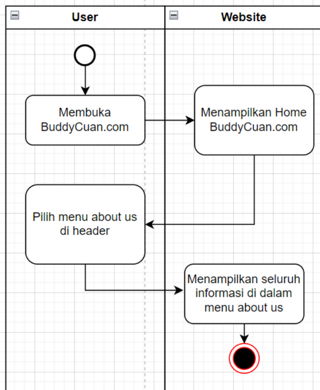
Gambar 3.2 Act Diagram Melihat Company Profile
