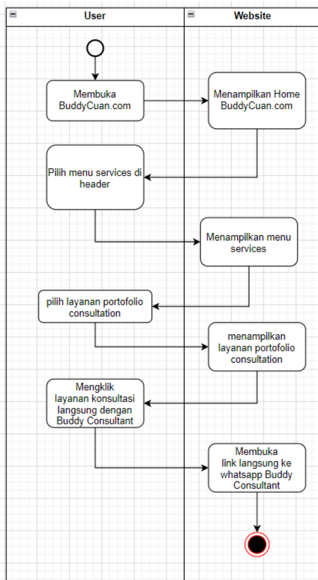
Gambar 3.8 Act Diagram Portofolio Consultation
