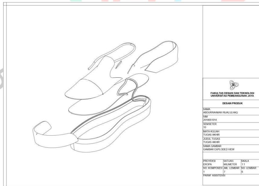
Lampiran 2. Exploded
