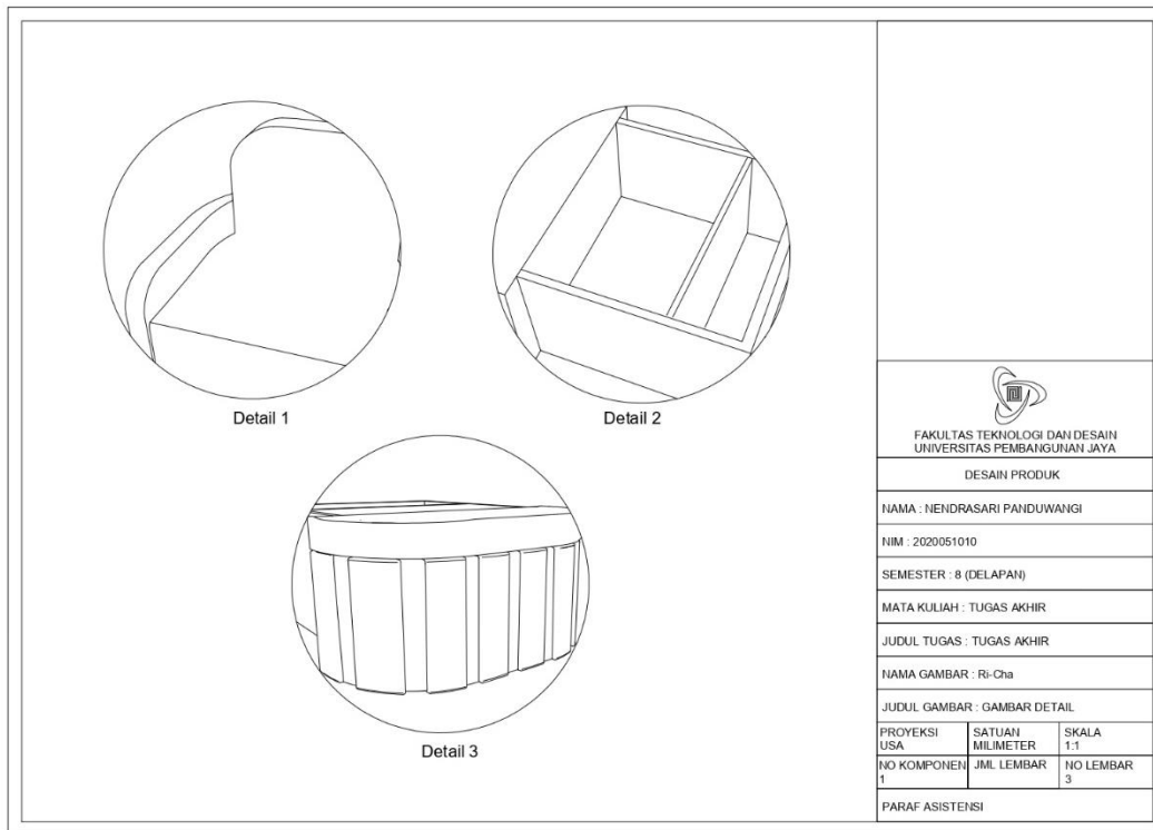
Lampiran 1 3 Gambar Detail
