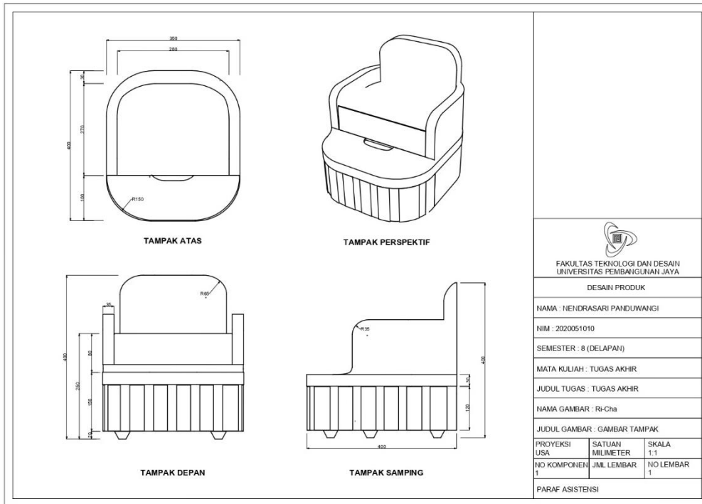
Lampiran 1 1 Gambar Tampak
