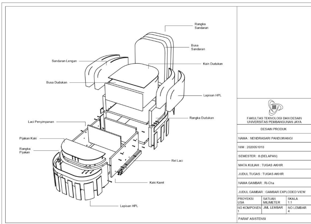
Lampiran 1 4 Gambar Exploded View
